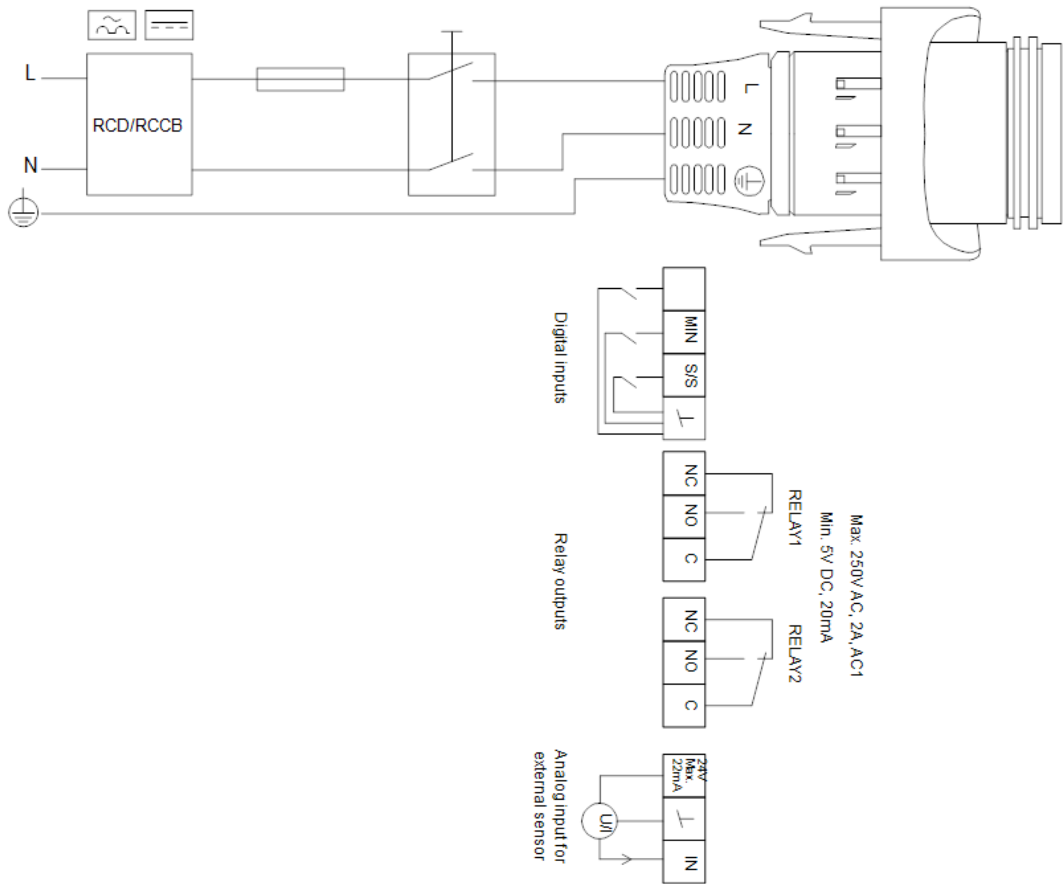
Example of plug-connected motor with mains switch, backup fuse and additional protection
